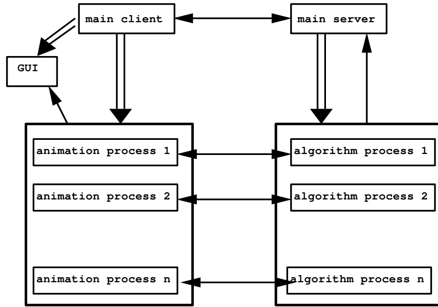
Figure 1: The VADE architecture
