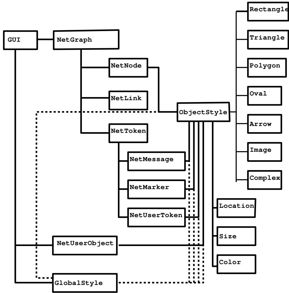
Figure 3: The structure of the animation classes
