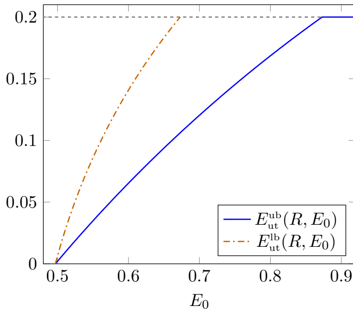
Figure 3: Upper tail double-exponential rate functions for the z -channel with crossover probability 0.001 and R = 0.2 .
