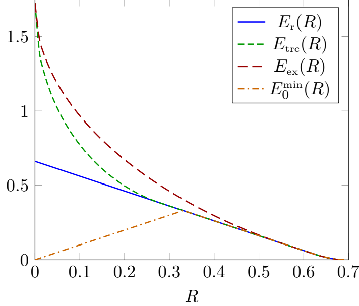
Figure 1: Various exponents for the z -channel with crossover probability 0.001.
