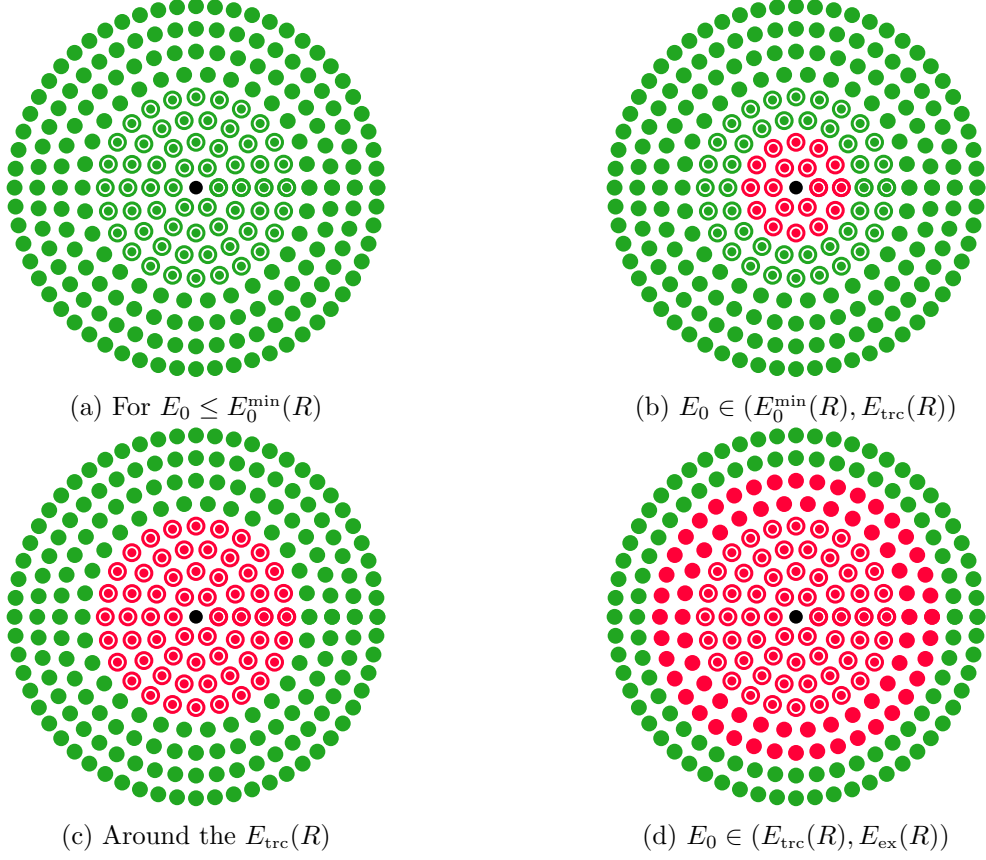
Figure 2: Typical populations for different E_0 values. The center is the true codeword and each concentric circle around it represents a conditional type class. The radii of the concentric circles represent distances between codewords, which are measured by the empirical conditional entropy (also proportional to the negative empirical mutual information), induced by the joint composition of the codewords. Dots denote the TP type classes and circle–dots represent the TE type classes. TP type classes are the sets of relatively distant codewords; they include all joint compositions Q_{XX'} with I_Q(X; X') \leq 2R . Red dots/circle–dots mean empty type classes. For larger E_0 values, the minimum distance between codewords increases.
