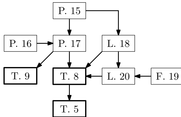
Figure 5. Roadmap for the proofs of the lower bounds (achievability). The used abbreviations are Lemma (L.), Proposition (P.), Theorem (T.) and Fact (F.). The result at the tail of an arrow is utilized to prove the result pointed by its head.
