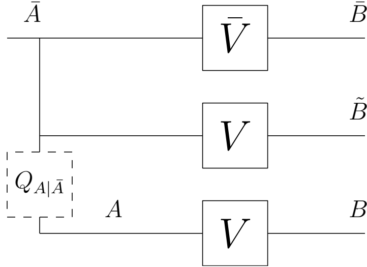
Figure 7. Channel model for a pair of “close” inputs
