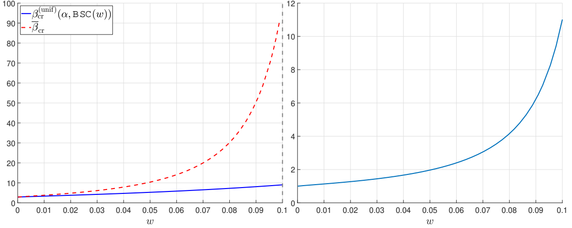
Figure 2. Comparison between [25, Theorem 1] and Prop. 13 for BSC. Left – \beta_{\text{cr}}^{(\text{unif})}(\alpha, \text{BSC}(w)) and \bar{\beta}_{\text{cr}} from [25, Theorem 1]. Right – the ratio \bar{\beta}_{\text{cr}}/\beta_{\text{cr}}^{(\text{unif})}(\alpha, \text{BSC}(w)) .
