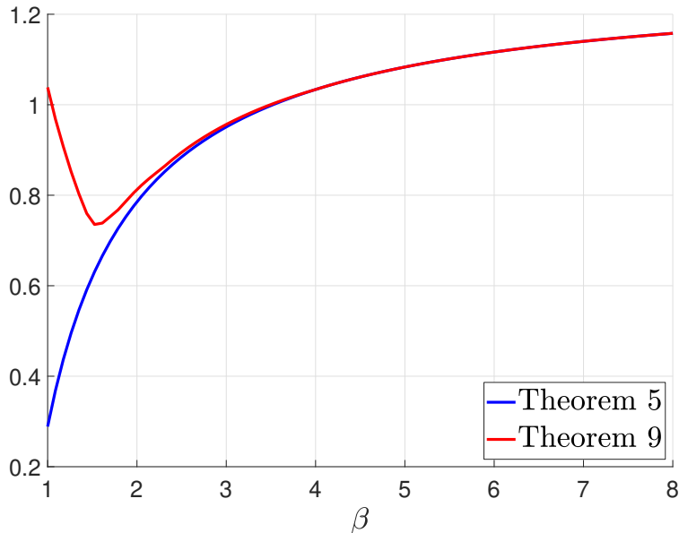
Figure 3. Upper and lower bounds on C(\text{DNA}(5, \beta, W_0)) as a function of \beta (in nats).
