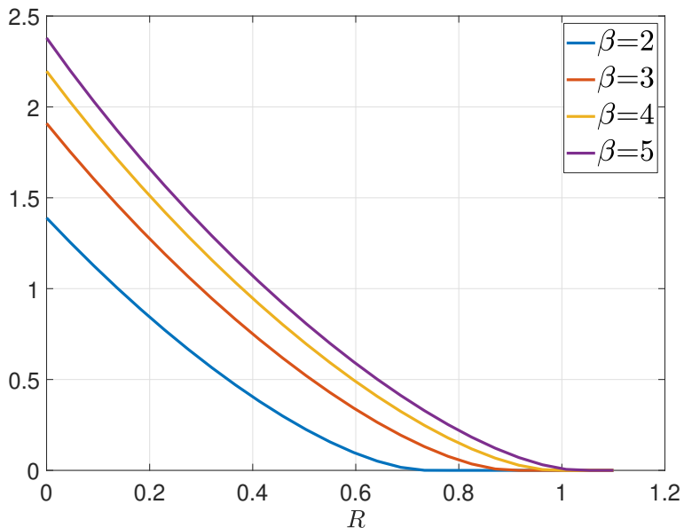
Figure 4. Lower bound on the reliability function E^*(R, \text{DNA}(5, \beta, W_0), \{M\}) as a function of R (in nats).
