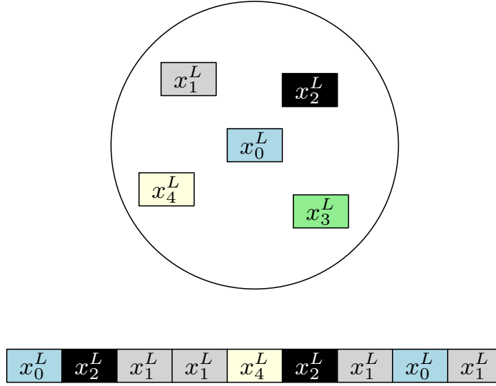
Figure 1. Illustration of a sampling event for M = 5 , and N = 9 . Here, U^9 = (0, 2, 1, 1, 4, 2, 1, 0, 1) , S^5 = (2, 4, 2, 0, 1) and Q^{10} = (1, 1, 2, 0, 1, 0, 0, 0, 0, 0) .
