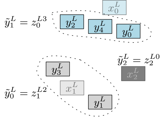
Figure 8. Illustration of permuted output clusters for M = 3 and N = 5 . Here, z_0^{L3} = (y_0^L, y_2^L, y_4^L) , z_1^{L2} = (y_1^L, y_3^L) and z_2^{L0} = () (is empty), while \tilde{u}^3 = (1, 0, 2) .
