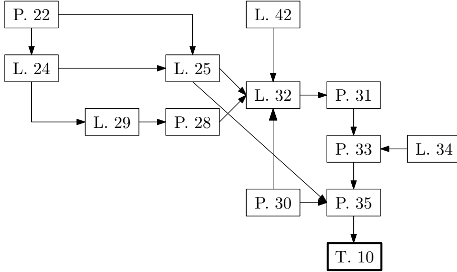
Figure 6. Roadmap for the proofs of the upper bound (converse). The used abbreviations and arrow interpretation are as in Fig. 5. .
