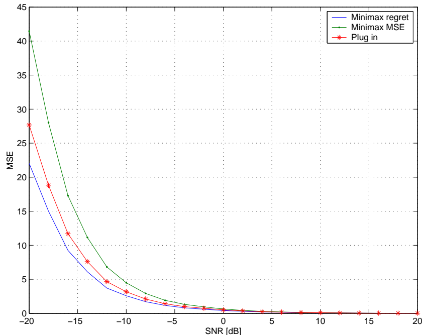
Figure 2: MSE in estimating \mathbf{x} from a noisy filtered version as a function of SNR using the minimax regret estimator, the minimax MSE estimator and the plug in MMSE estimator matched to the estimated covariance matrix.
