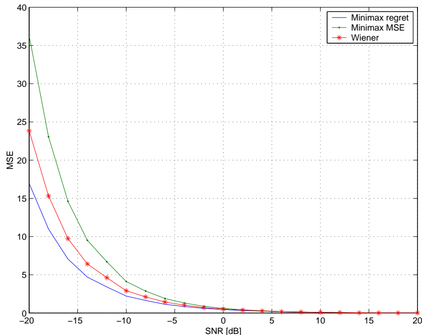
Figure 1: MSE in estimating \mathbf{x} as a function of SNR using the minimax regret estimator, the minimax MSE estimator and the plug in MMSE estimator matched to the estimated covariance matrix.
