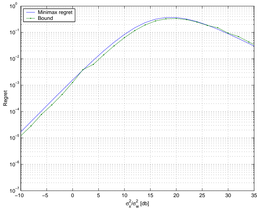
Figure 3: Worst-case regret in estimating x as a function of SNR using the linear minimax regret estimator, and the bound on the smallest worst-case regret attainable using a third-order estimator.
