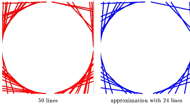
Figure 3: Annulus Distribution
