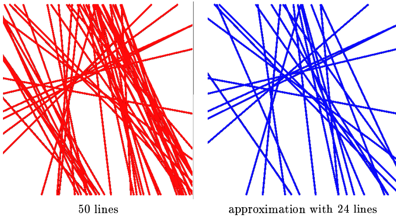
Figure 5: Clusnorm Distribution
