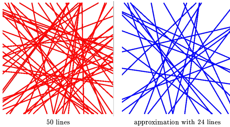
Figure 2: Uniform Distribution
