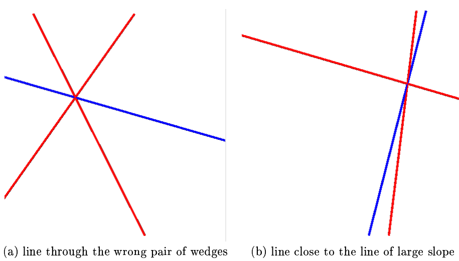
Figure 1: Midpoint replacement
