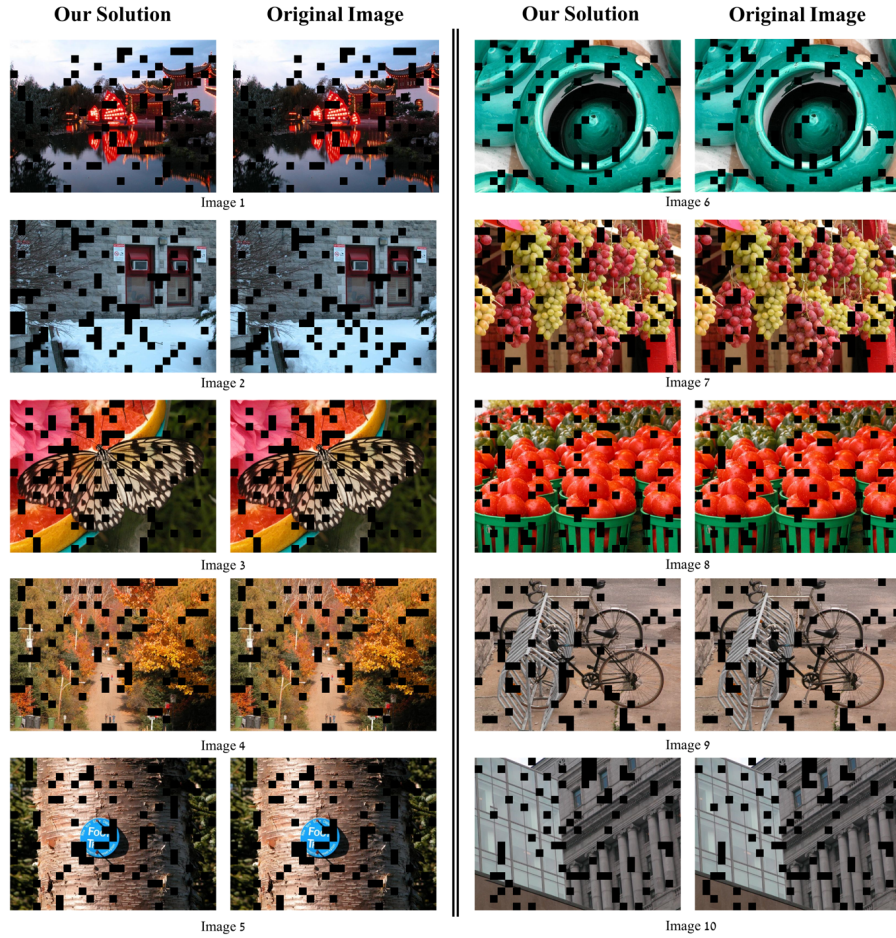
Figure 6. 10 puzzles out of 20 from the dataset of [17]
